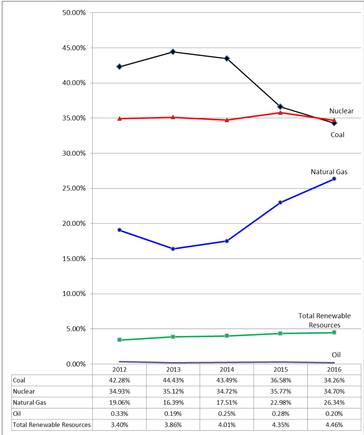
Figure 1: PJM System Fuel Mix 2012 - 2016
